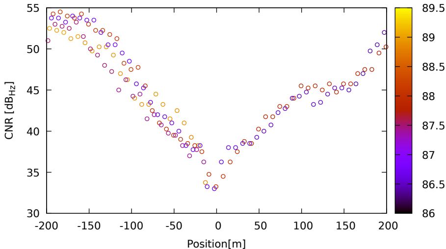
CNR vs position for E12 (E5) on LeicaGS18 - DOY 263 jam. 1
