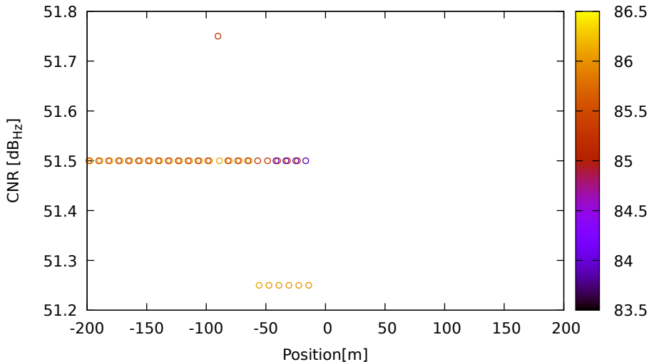
CNR vs position for E12 (E5a) on LeicaGS18 - DOY 263 jam. 2
