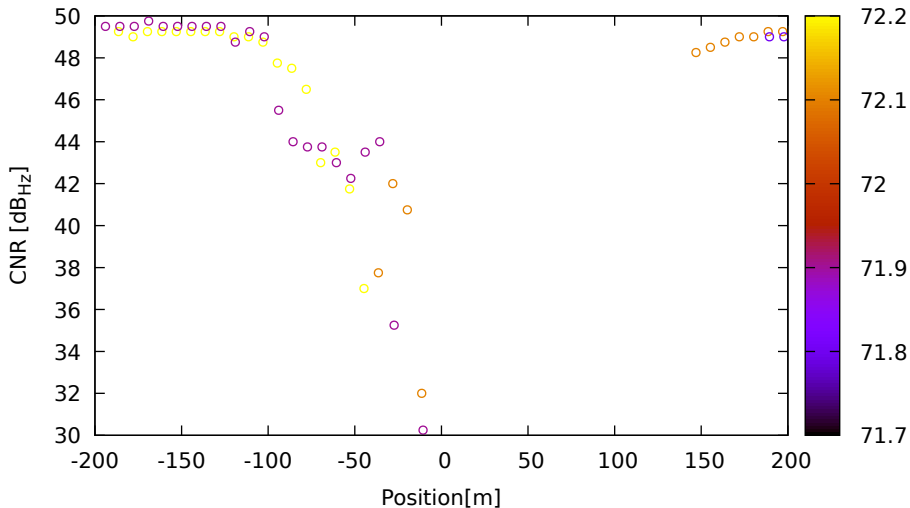
CNR vs position for E19 (E1) on LeicaGS18 - DOY 263 jam. 3
