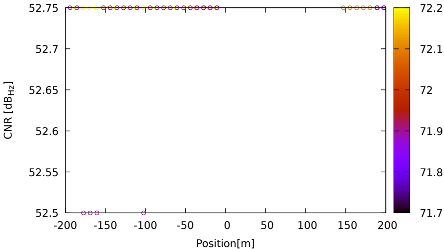
CNR vs position for E19 (E5) on LeicaGS18 - DOY 263 jam. 3
