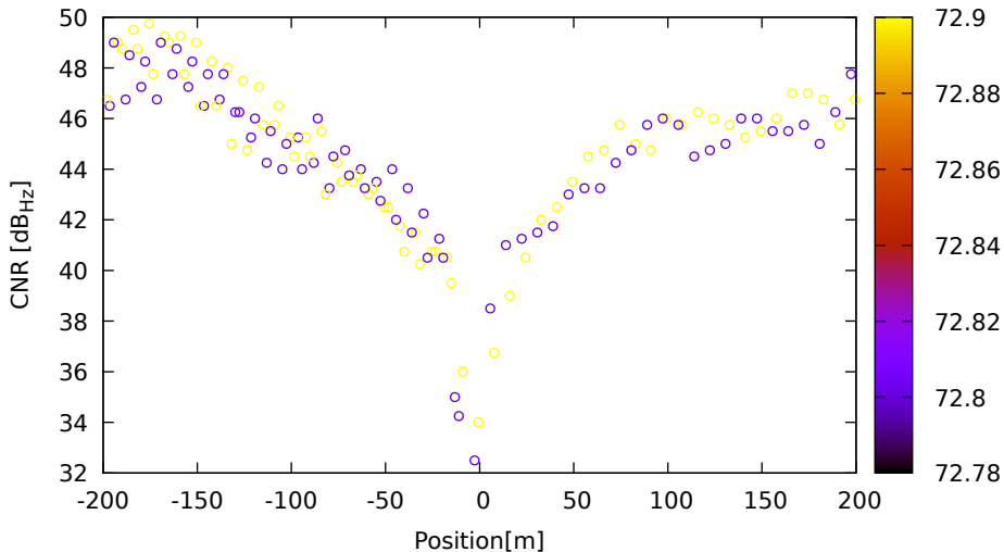
CNR vs position for E19 (E5b) on LeicaGS18 - DOY 263 jam. 1
