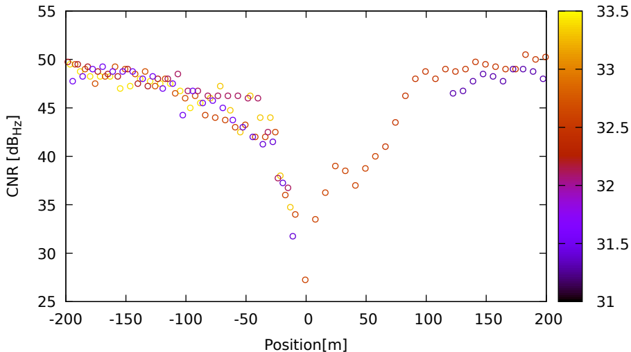
CNR vs position for E33 (E1) on LeicaGS18 - DOY 263 jam. 1
