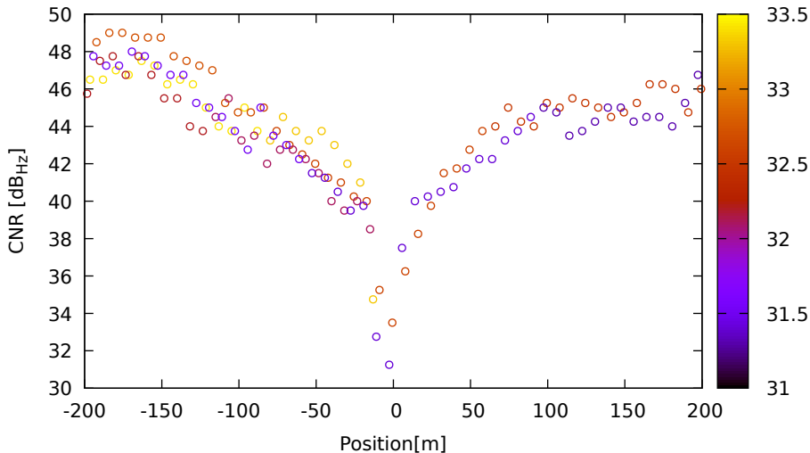
CNR vs position for E33 (E5b) on LeicaGS18 - DOY 263 jam. 1
