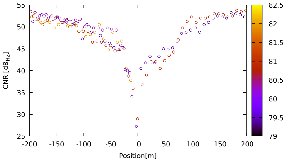
CNR vs position for G01 (L2) on LeicaGS18 - DOY 263 jam. 1
