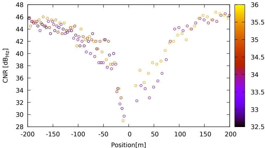
CNR vs position for G04 (L1) on LeicaGS18 - DOY 263 jam. 1
