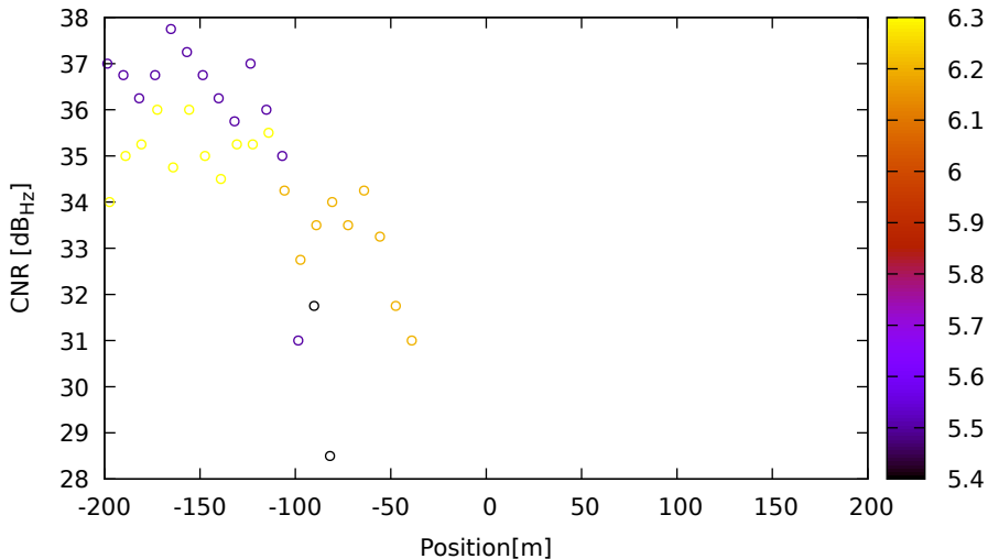
CNR vs position for G08 (L2) on LeicaGS18 - DOY 263 jam. 2
