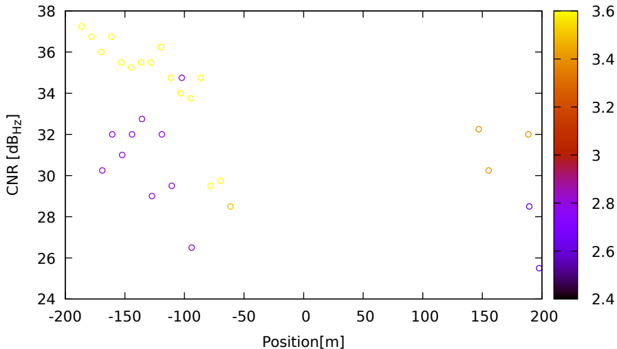
CNR vs position for G08 (L2) on LeicaGS18 - DOY 263 jam. 3
