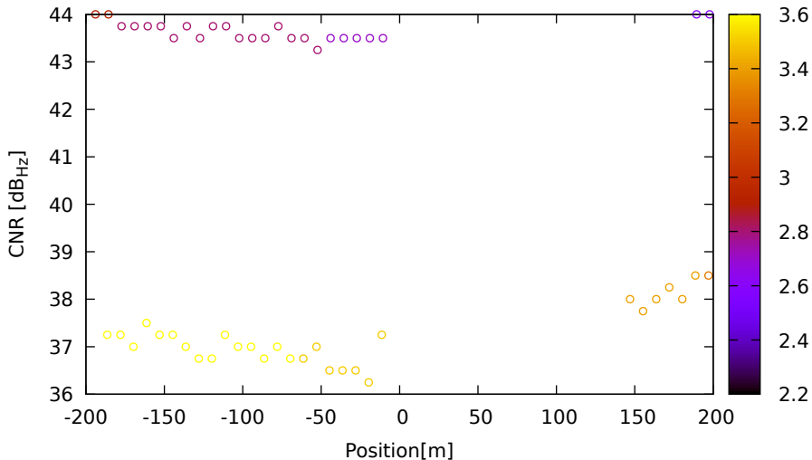
CNR vs position for G08 (L5) on LeicaGS18 - DOY 263 jam. 3
