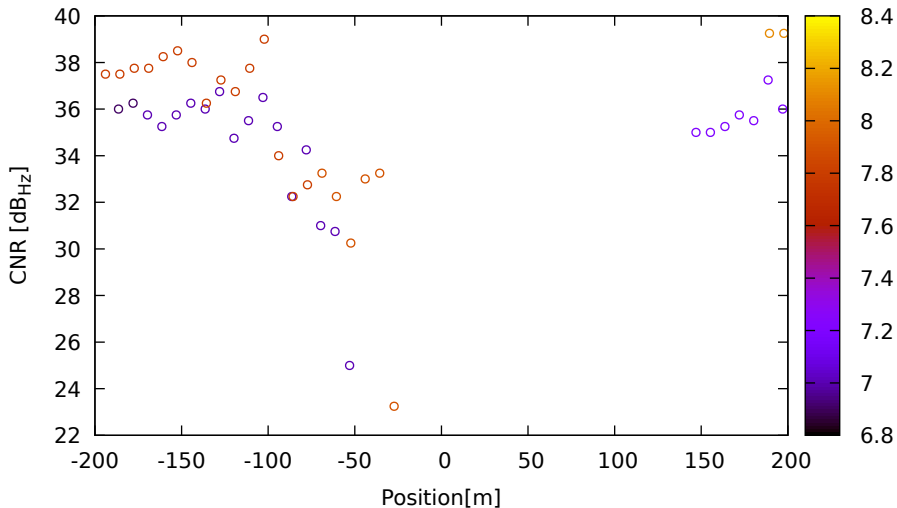
CNR vs position for G09 (L2) on LeicaGS18 - DOY 263 jam. 3
