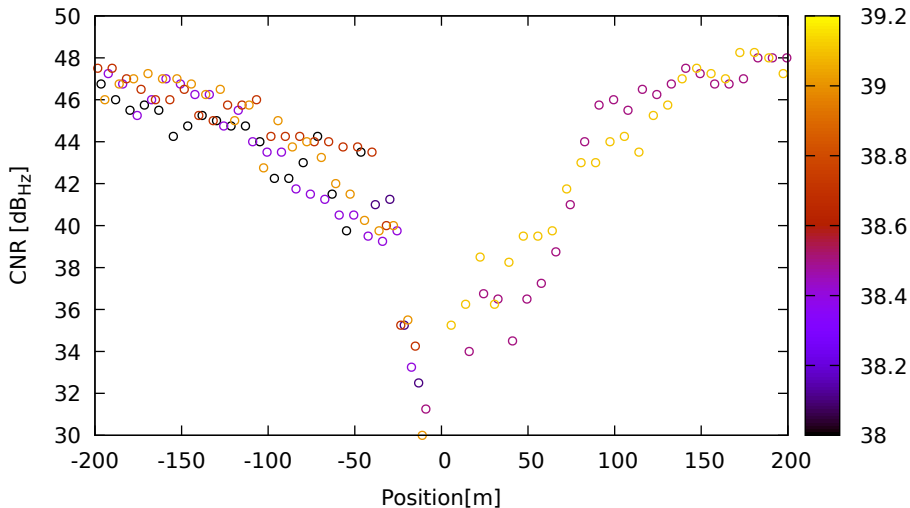
CNR vs position for G17 (L1) on LeicaGS18 - DOY 263 jam. 1
