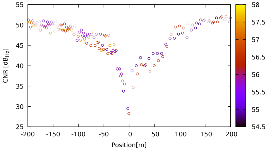
CNR vs position for G21 (L1) on LeicaGS18 - DOY 263 jam. 1
