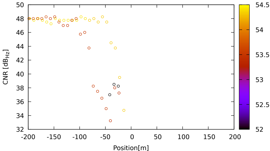
CNR vs position for G21 (L2) on LeicaGS18 - DOY 263 jam. 2
