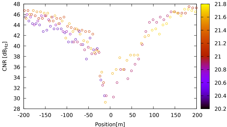
CNR vs position for G31 (L1) on LeicaGS18 - DOY 263 jam. 1
