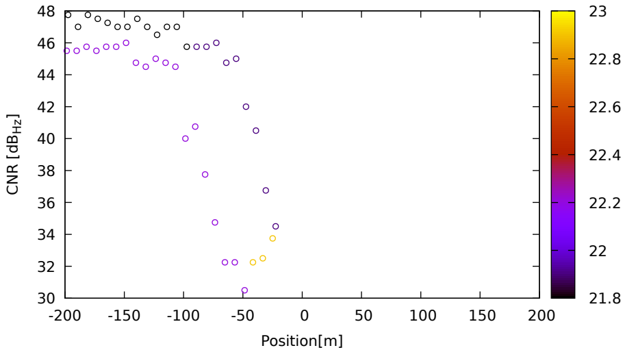
CNR vs position for G31 (L2) on LeicaGS18 - DOY 263 jam. 2
