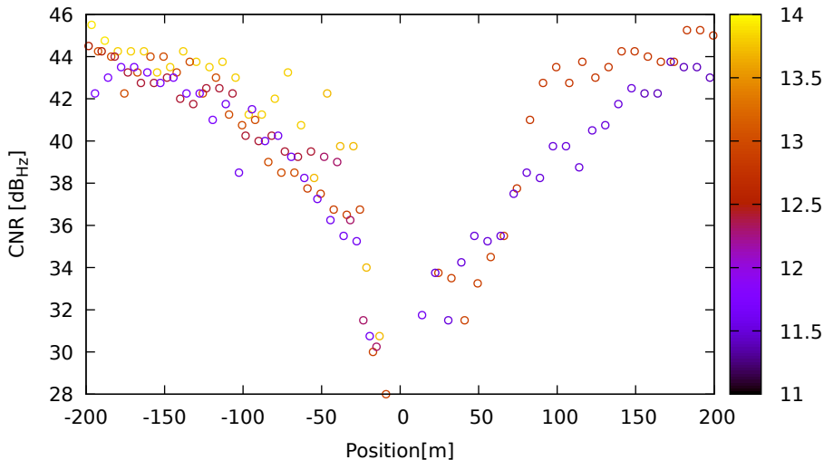
CNR vs position for G32 (L1) on LeicaGS18 - DOY 263 jam. 1
