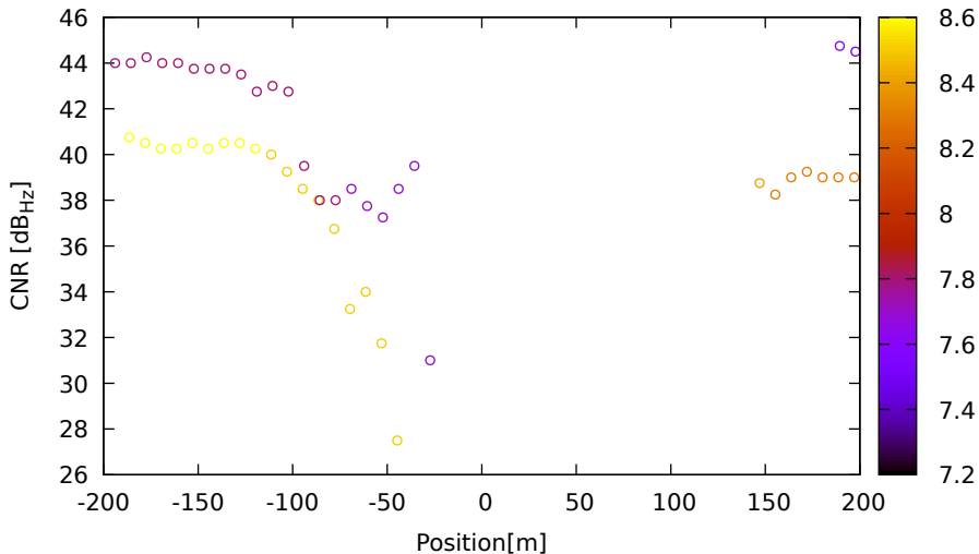
CNR vs position for G32 (L1) on LeicaGS18 - DOY 263 jam. 3
