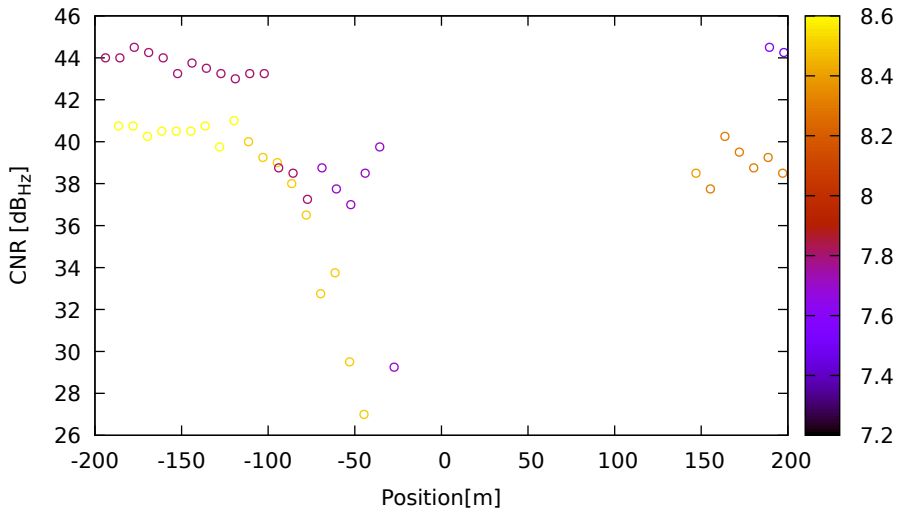
CNR vs position for G32 (L2) on LeicaGS18 - DOY 263 jam. 3
