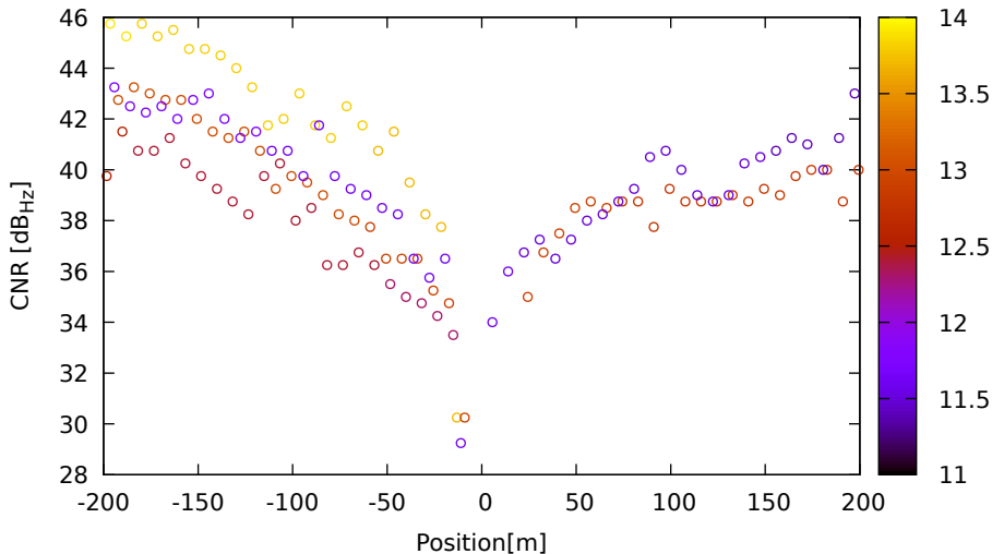
CNR vs position for G32 (L5) on LeicaGS18 - DOY 263 jam. 1
