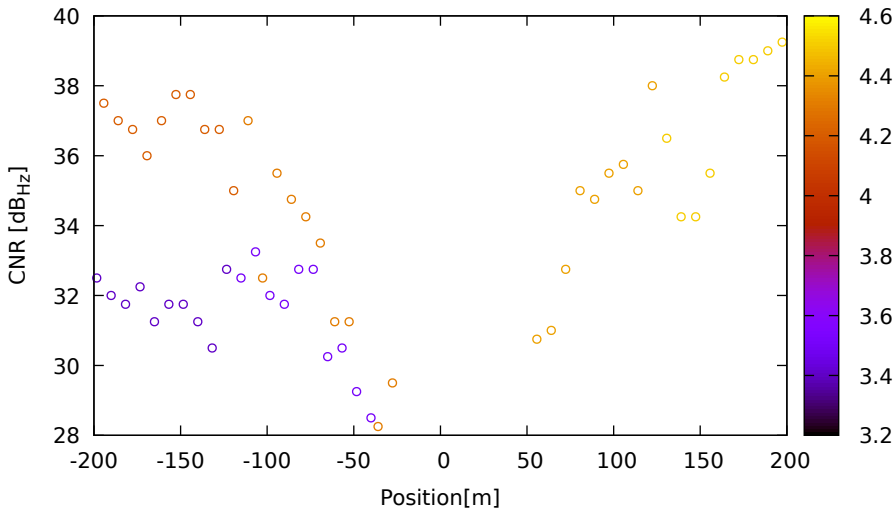
CNR vs position for R03 (G1) on LeicaGS18 - DOY 263 jam. 1
