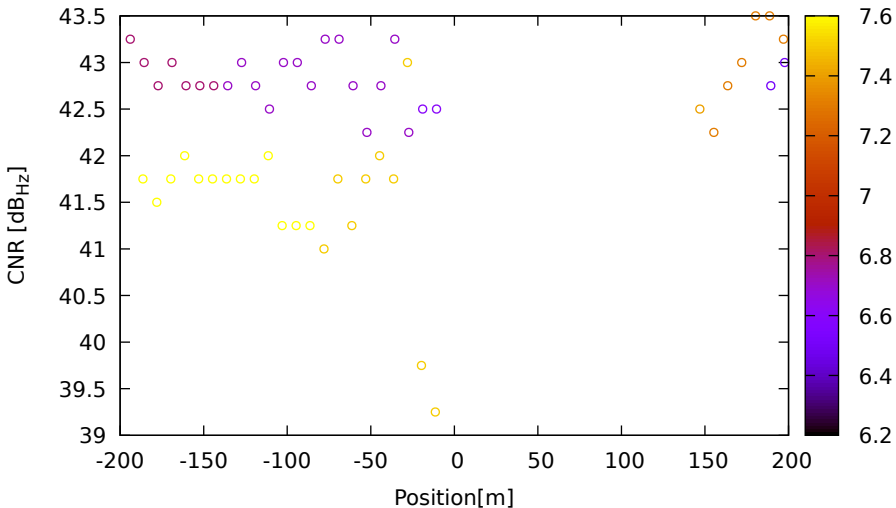
CNR vs position for R08 (G1) on LeicaGS18 - DOY 263 jam. 3
