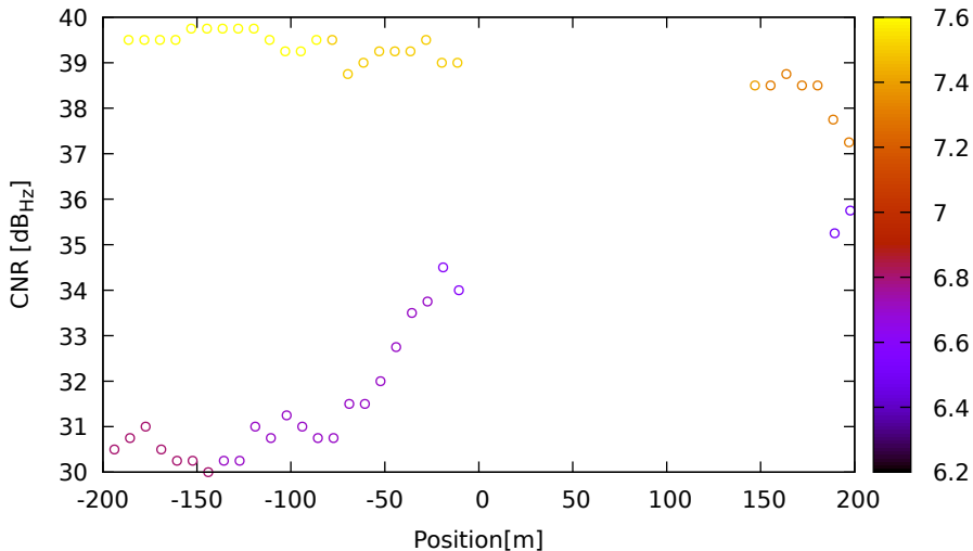
CNR vs position for R08 (G2) on LeicaGS18 - DOY 263 jam. 3
