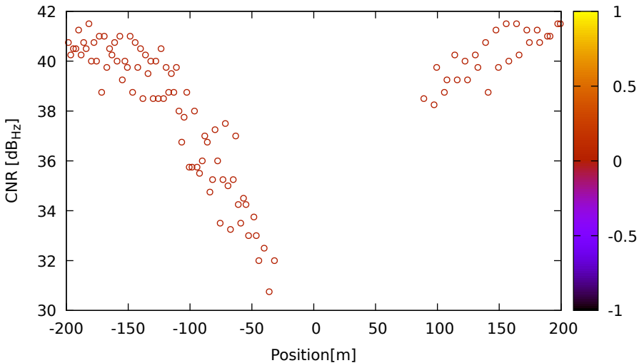
CNR vs position for R09 (G2) on LeicaGS18 - DOY 263 jam. 1
