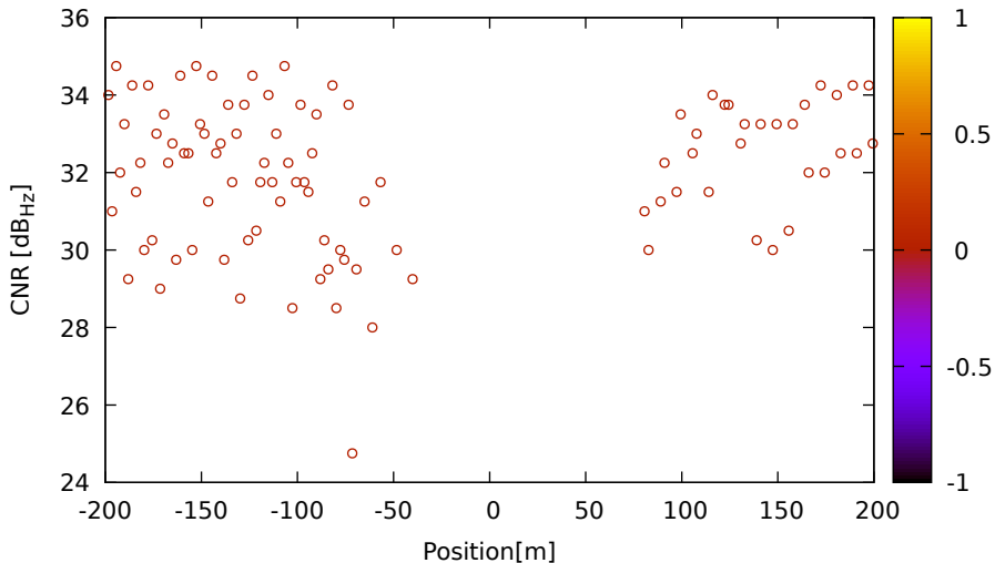
CNR vs position for R10 (G1) on LeicaGS18 - DOY 263 jam. 1
