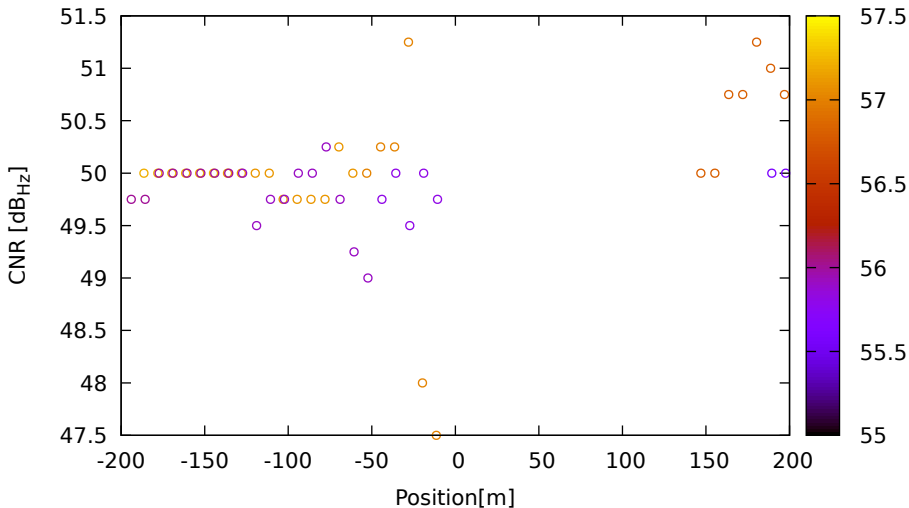
CNR vs position for R24 (G1) on LeicaGS18 - DOY 263 jam. 3
