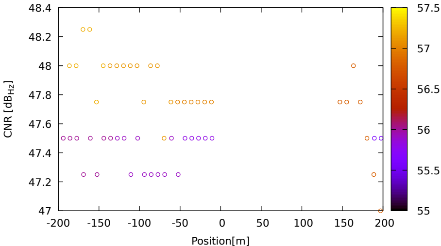
CNR vs position for R24 (G2) on LeicaGS18 - DOY 263 jam. 3
