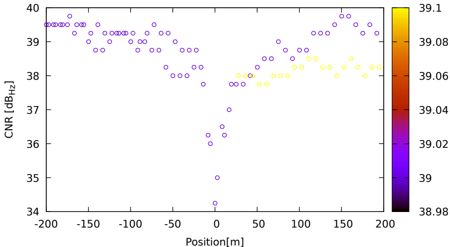
CNR vs position for C09 (B1) on SamsungS20 - DOY 263 jam. 3
