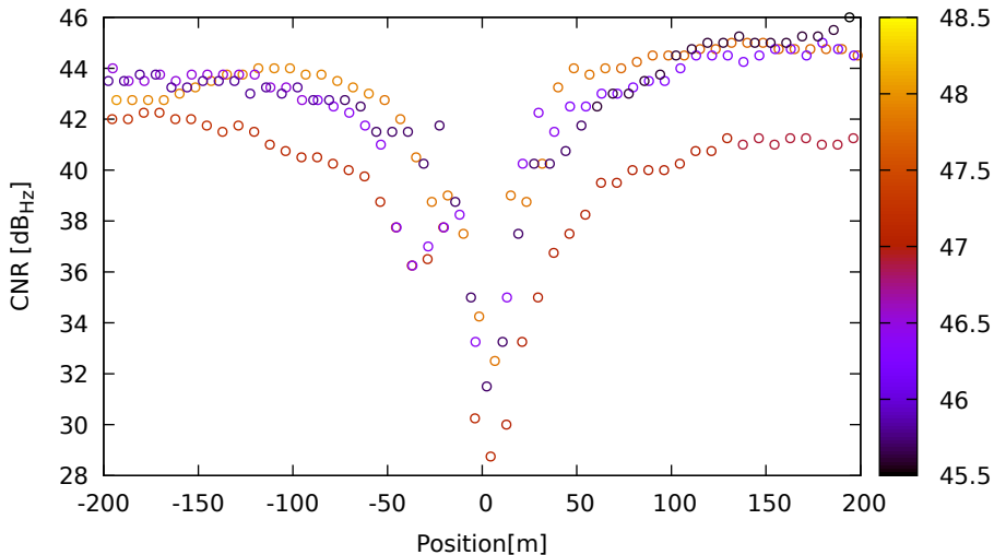
CNR vs position for C21 (B1) on SamsungS20 - DOY 263 jam. 1
