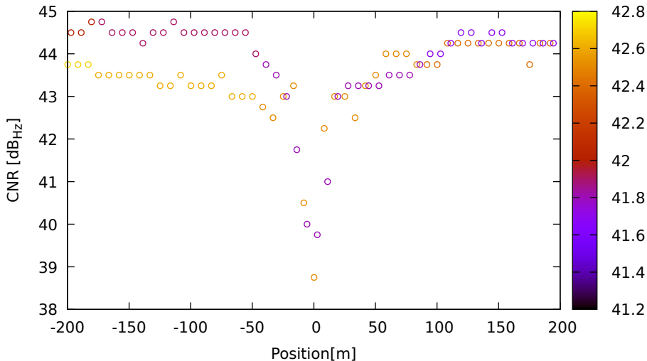
CNR vs position for C21 (B1) on SamsungS20 - DOY 263 jam. 3
