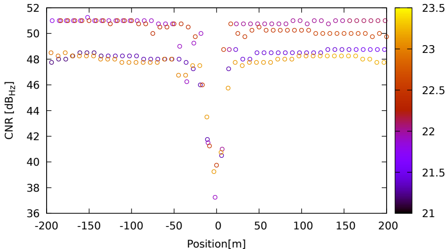
CNR vs position for C28 (B1) on SamsungS20 - DOY 263 jam. 2
