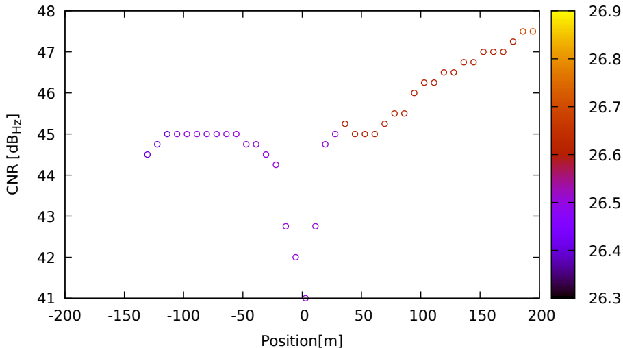
CNR vs position for C33 (B1) on SamsungS20 - DOY 263 jam. 3
