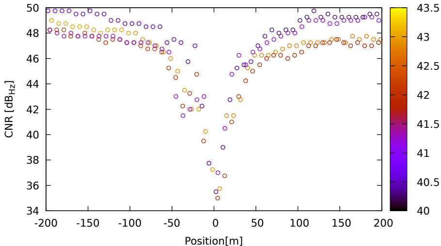
CNR vs position for C34 (B1) on SamsungS20 - DOY 263 jam. 1
