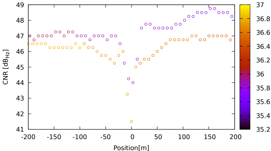
CNR vs position for C34 (B1) on SamsungS20 - DOY 263 jam. 3
