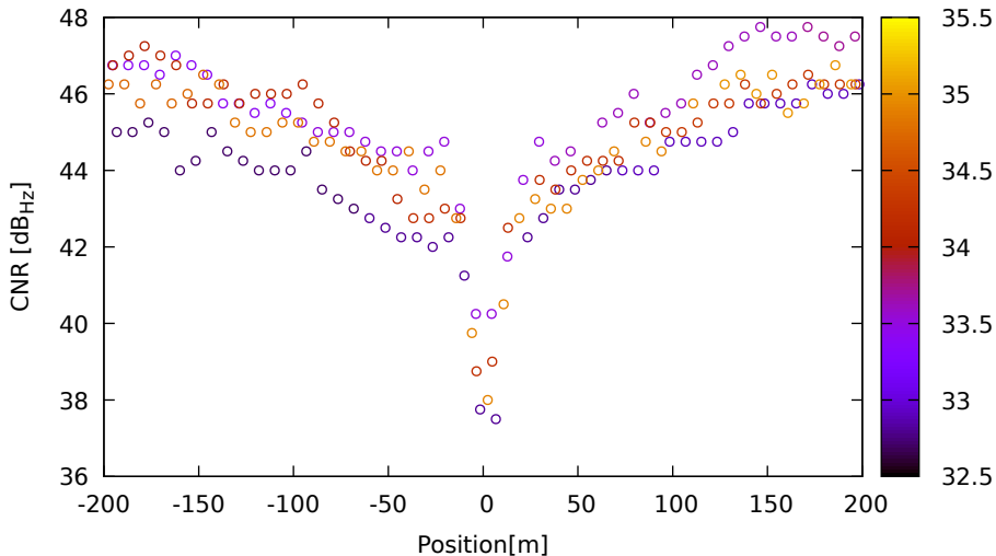
CNR vs position for E04 (E1) on SamsungS20 - DOY 263 jam. 1
