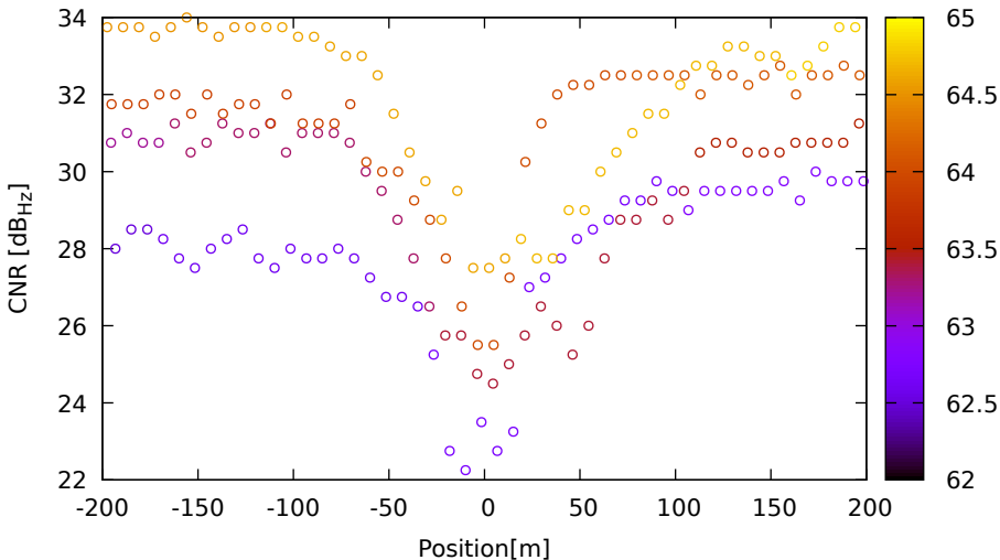
CNR vs position for E10 (E5a) on SamsungS20 - DOY 263 jam. 1
