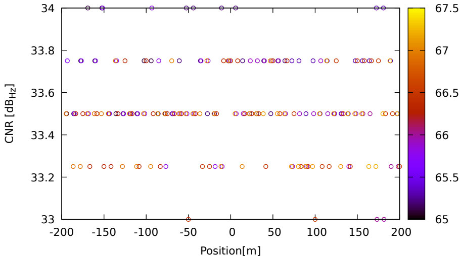
CNR vs position for E10 (E5a) on SamsungS20 - DOY 263 jam. 2
