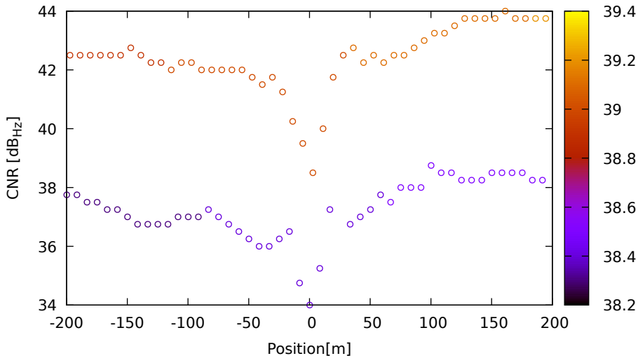
CNR vs position for E11 (E1) on SamsungS20 - DOY 263 jam. 3
