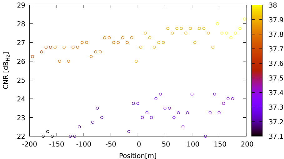
CNR vs position for E11 (E5a) on SamsungS20 - DOY 263 jam. 2
