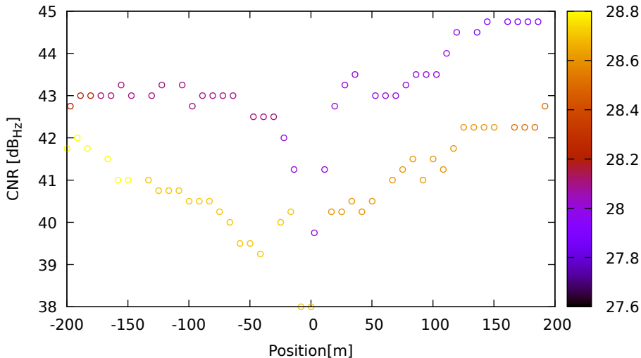
CNR vs position for E33 (E1) on SamsungS20 - DOY 263 jam. 3
