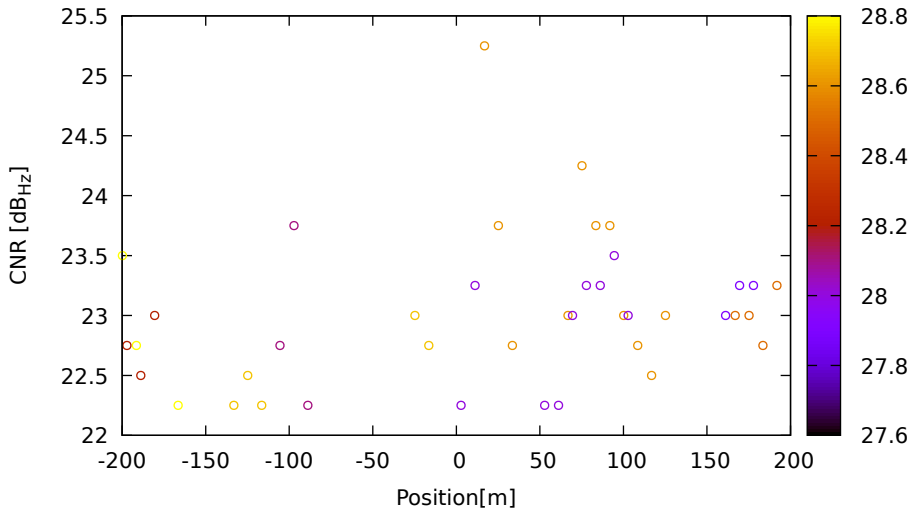
CNR vs position for E33 (E5a) on SamsungS20 - DOY 263 jam. 3
