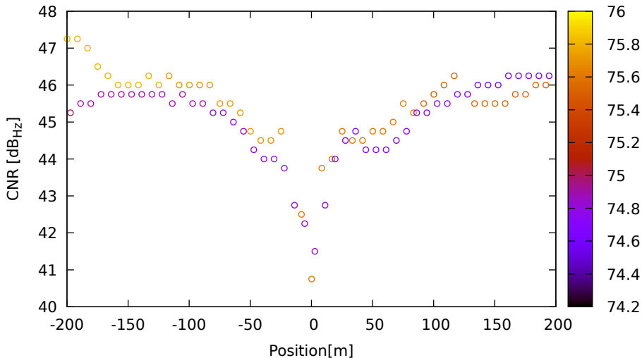
CNR vs position for G01 (L1) on SamsungS20 - DOY 263 jam. 3
