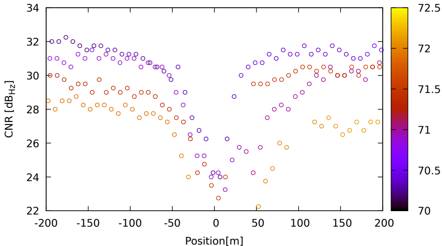
CNR vs position for G03 (L5) on SamsungS20 - DOY 263 jam. 1
