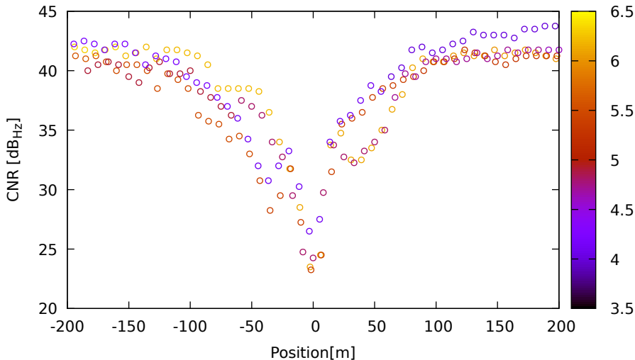
CNR vs position for G08 (L1) on SamsungS20 - DOY 263 jam. 2
