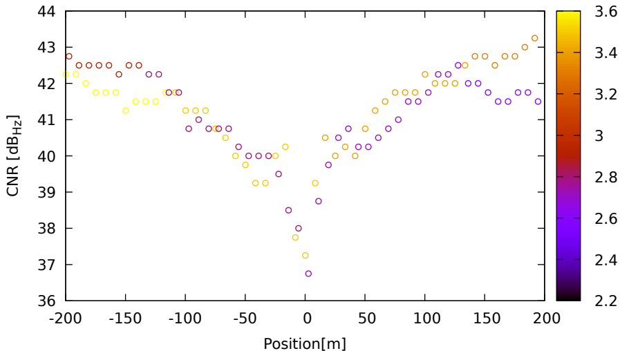
CNR vs position for G08 (L1) on SamsungS20 - DOY 263 jam. 3
