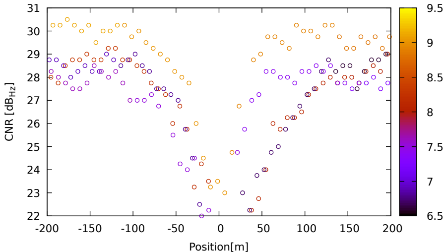
CNR vs position for G08 (L5) on SamsungS20 - DOY 263 jam. 1
