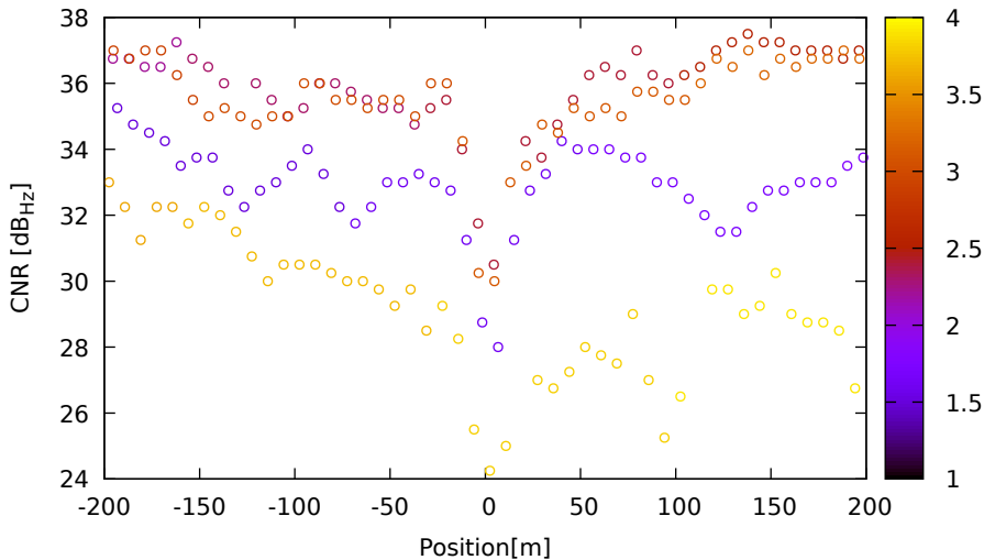
CNR vs position for G09 (L1) on SamsungS20 - DOY 263 jam. 1
