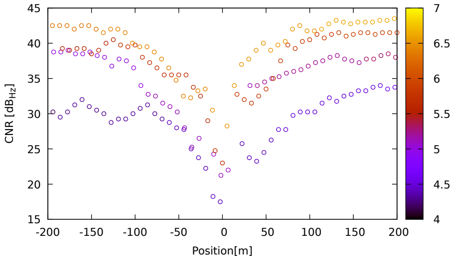
CNR vs position for G09 (L1) on SamsungS20 - DOY 263 jam. 2
